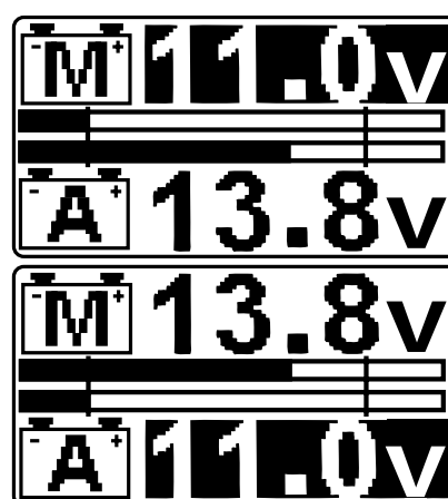
Fig. 3 - Under voltage indication
